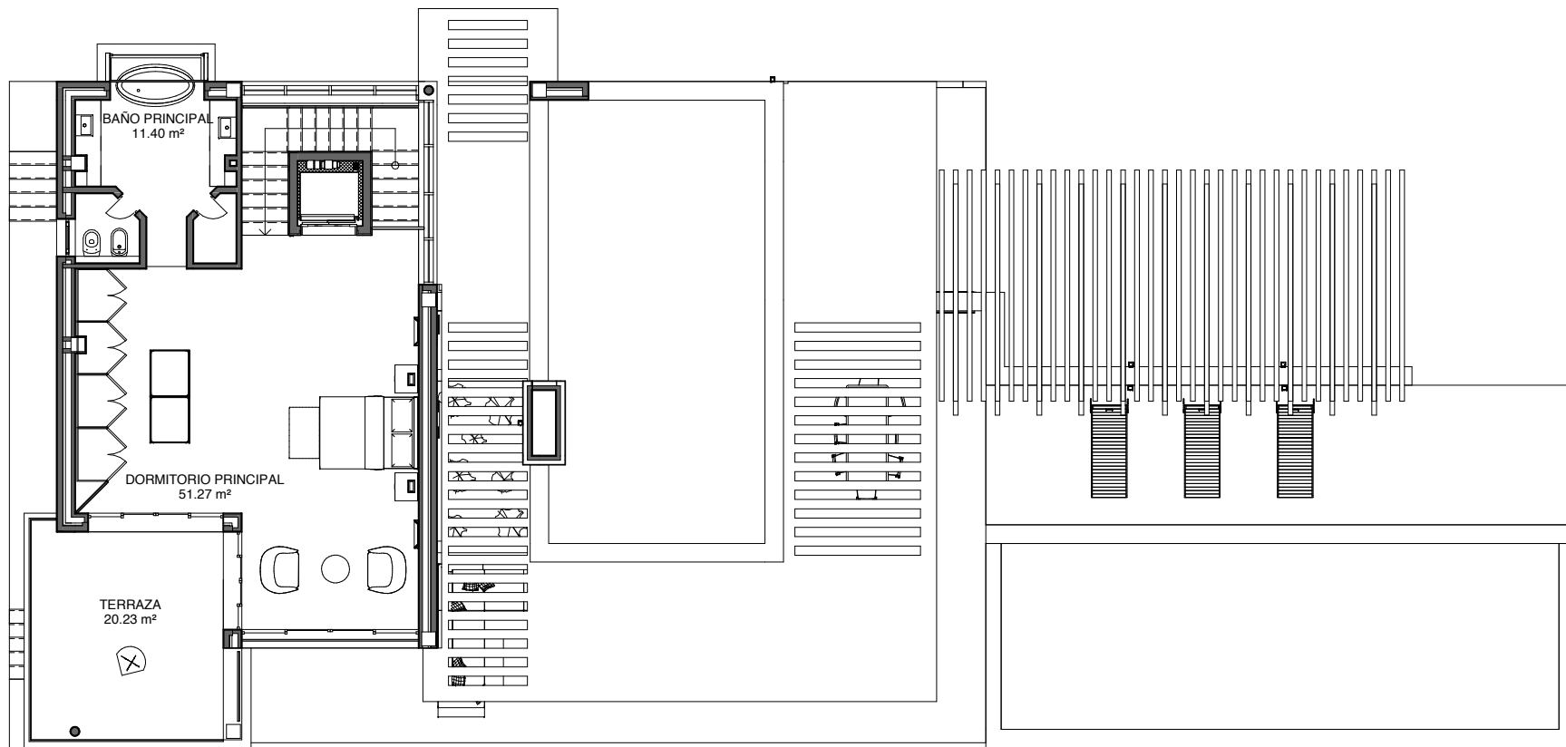
PLANTA ALTA FIRST FLOOR
