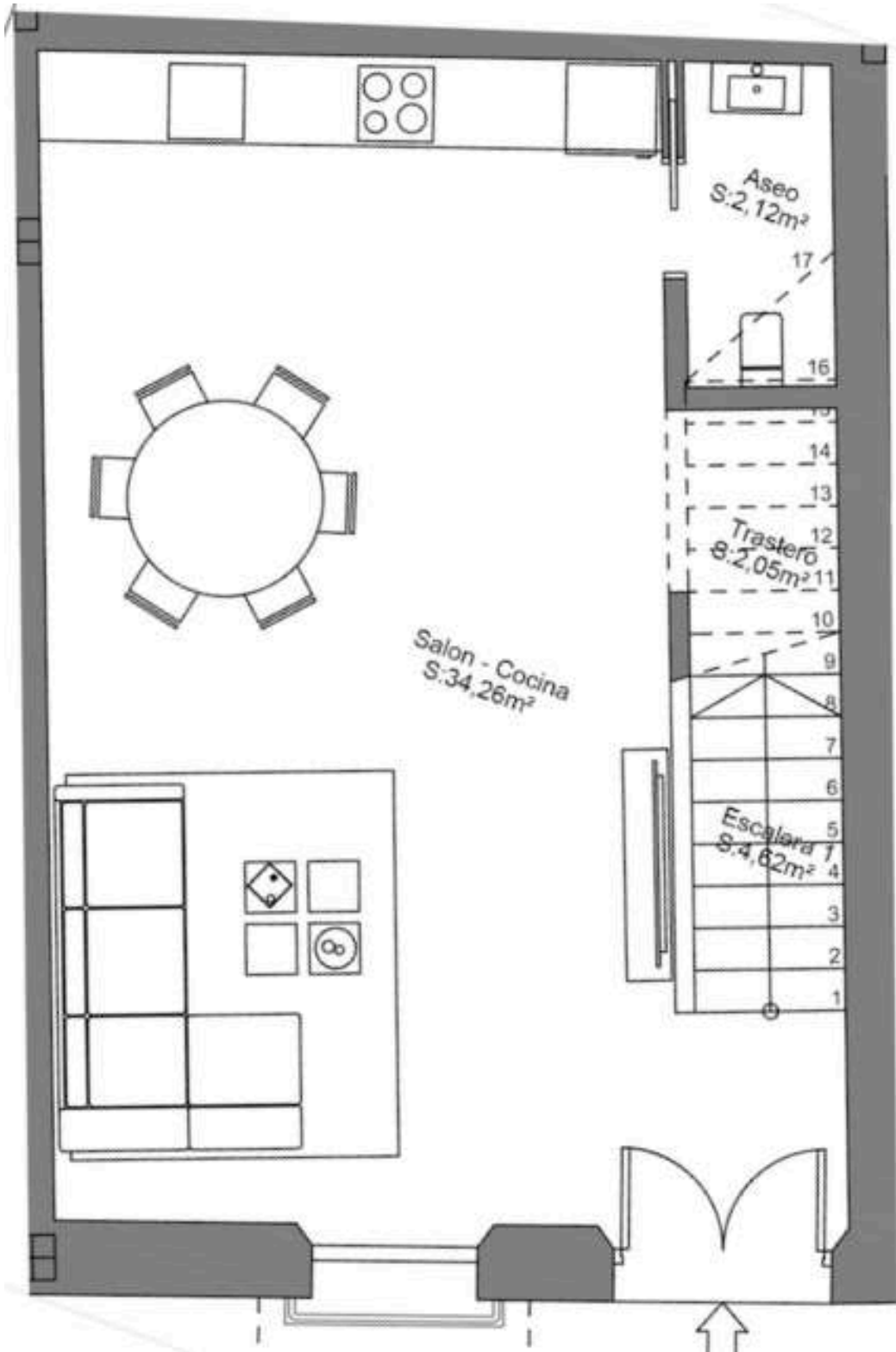
GROUND FLOOR
