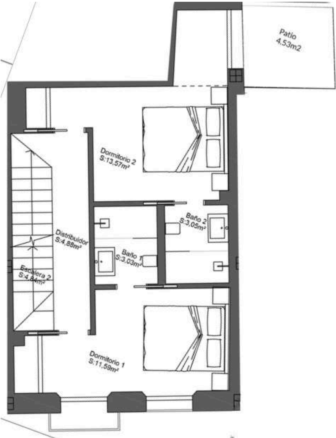
FIRST FLOOR
