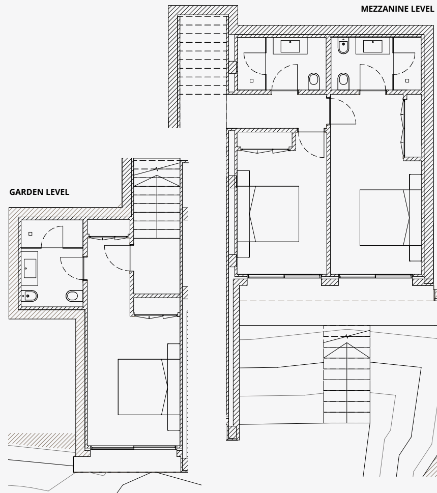
VILLA TOMILLO GARDEN + MEZZANINE
