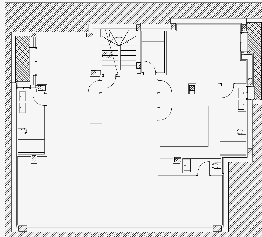
VILLA MENTA BASEMENT
