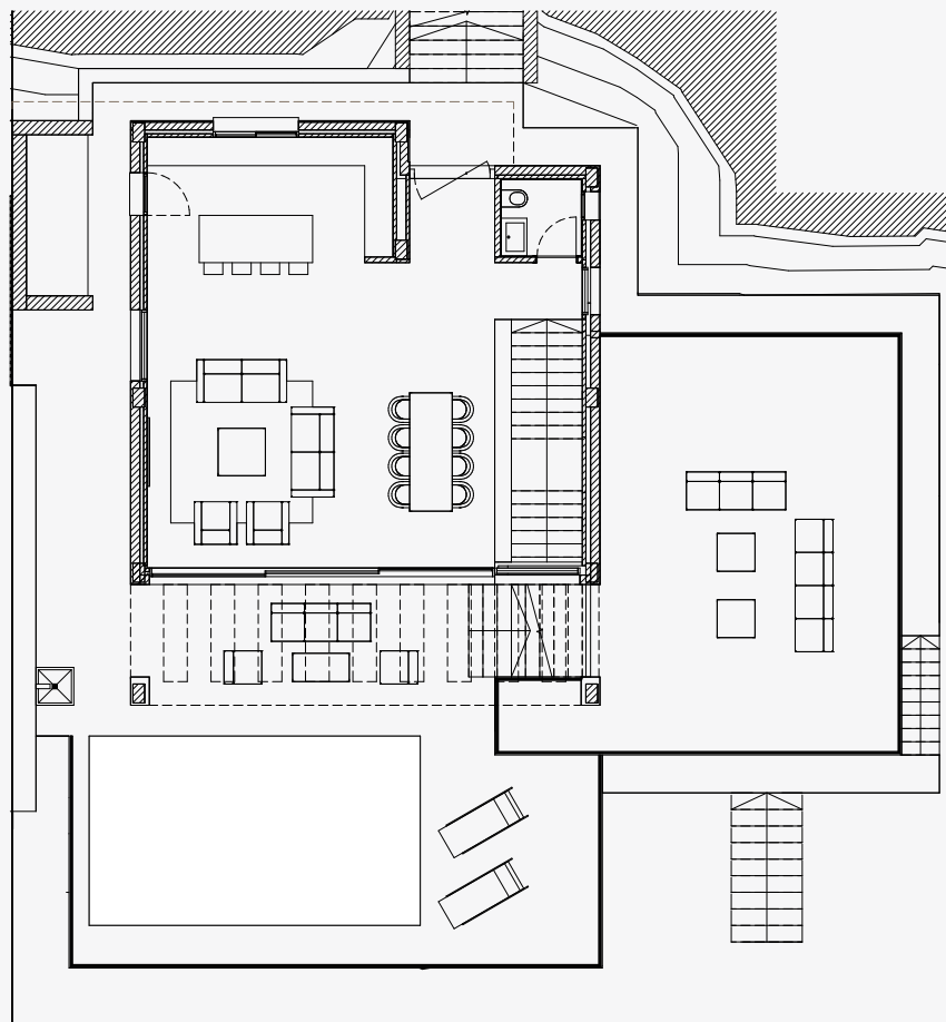
VILLA TOMILLO GROUND FLOOR
