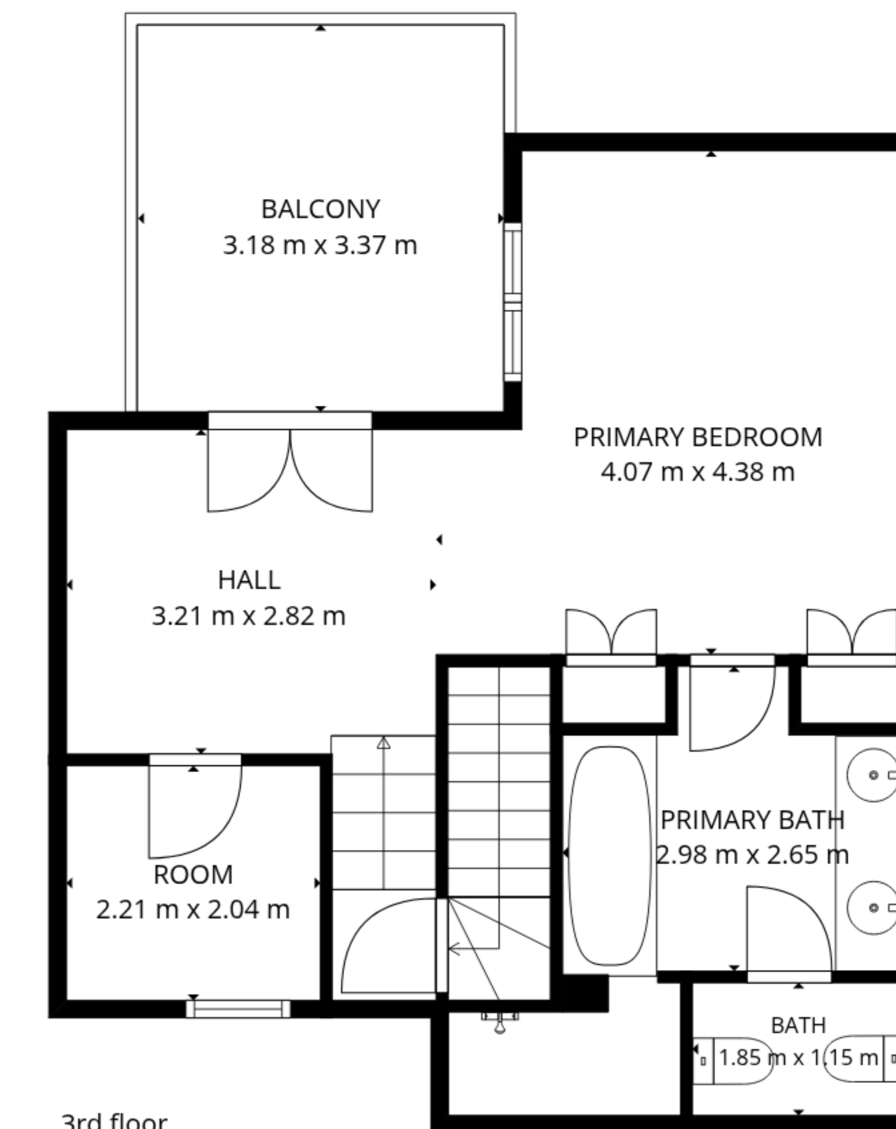
3rd floor
