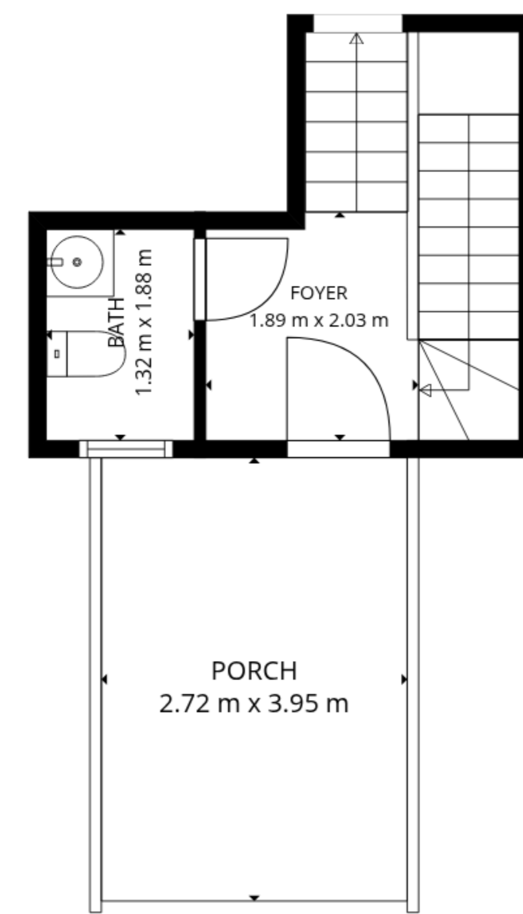
1st floor
