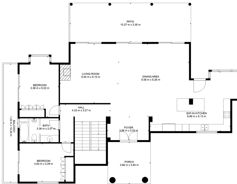
FLOOR 2
